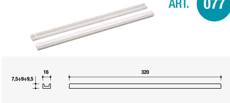
Corrente per cassetti con fermo dx e sx Running guide right or left for drawers with stopping device
